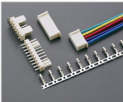
250H Series Pitch:2.5mm Page:113-115
